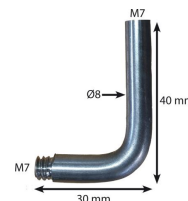
Raccord coudé - côtes
