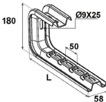
Equerre universelle CWU - sch  ma technique
